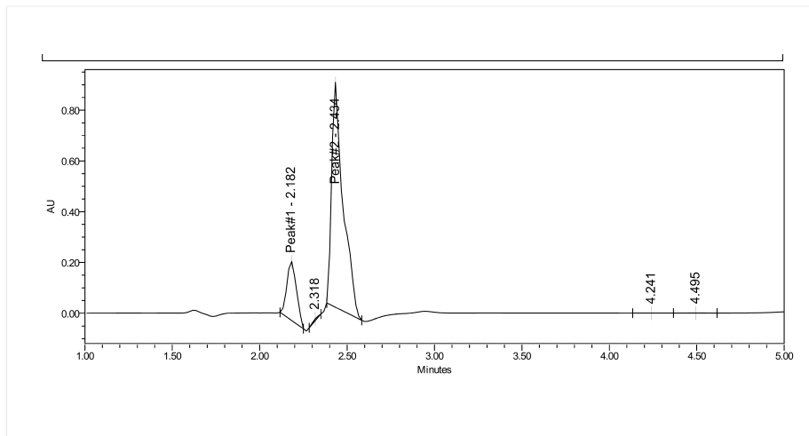
Fig. 1 - HPLC-UV Chromatogram at 214nm
